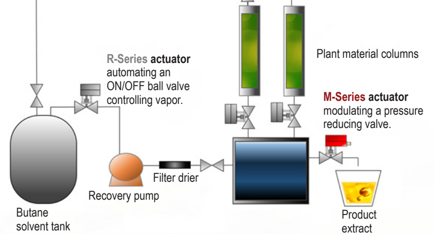
Simplified schematic of a closed loop butane extractor with Hanbay ex-proof electric actuators.
