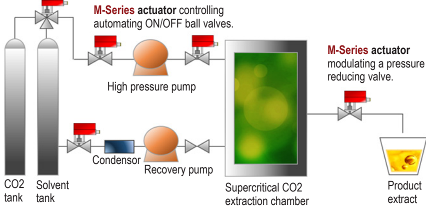
Simplified schematic of a superficial CO2 extractor with Hanbay electric actuators.
