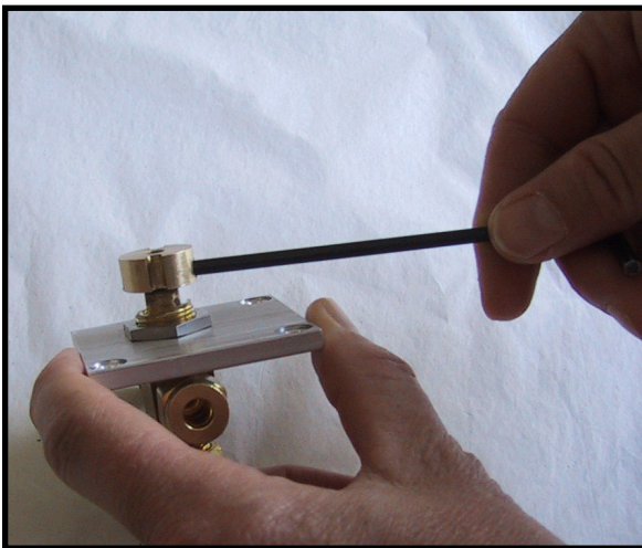
Mounting the Valve lever
