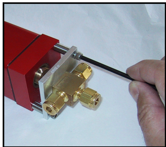
Mounting assembly to actuator
